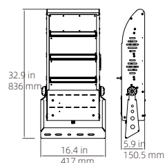
630W Weight: 16.8 KG Remove driver: 13.3 KG
