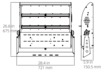
840W Weight: 23.5 KG Remove driver: 18.2 KG
