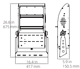
420W Weight: 13.9 KG Remove driver: 11.3 KG
