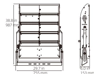
1600W Weight: 33.6 KG Remove driver: 26.6 KG
