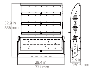
1060W /1260W Weight: 28.5 KG Remove driver: 21.5 KG
